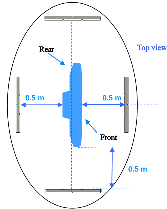
Figure B.4.1.3.1. Measurement geometry for band I and band II.
