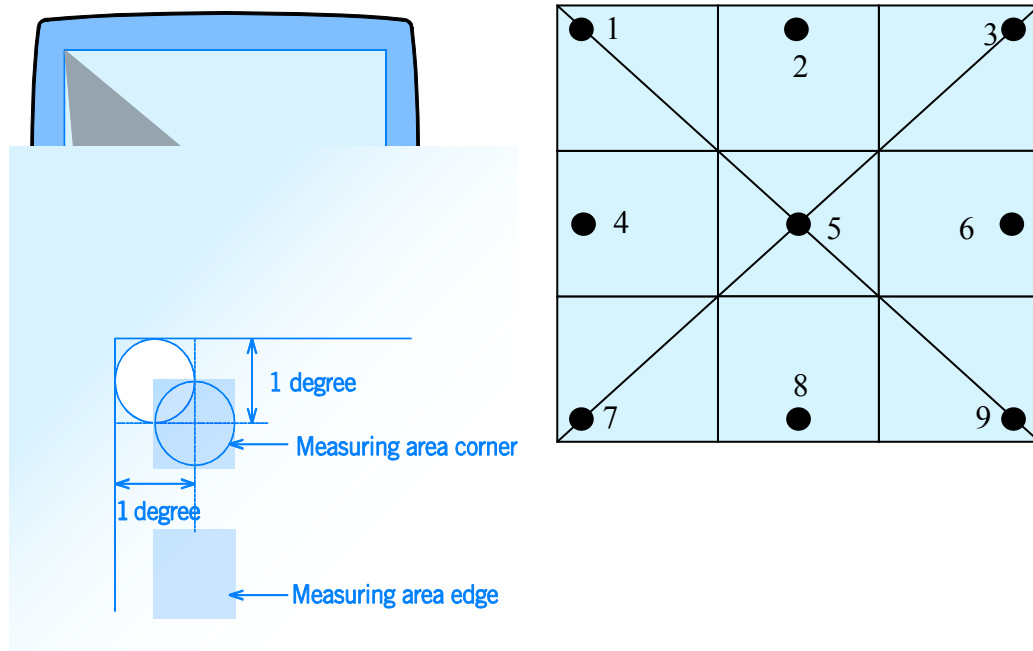
Figure B.2.2.2.1. Measurement positions for the measurement of luminance and colour uniformity.
