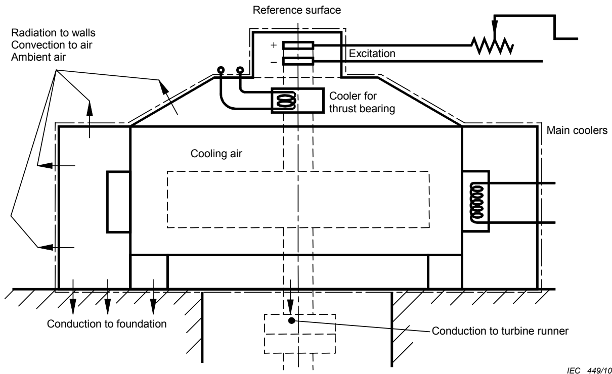
Figure 2 – Reference surface
