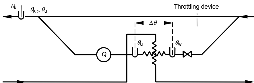
Figure 6 – Parallel piping
